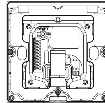
4 BACK VIEW
